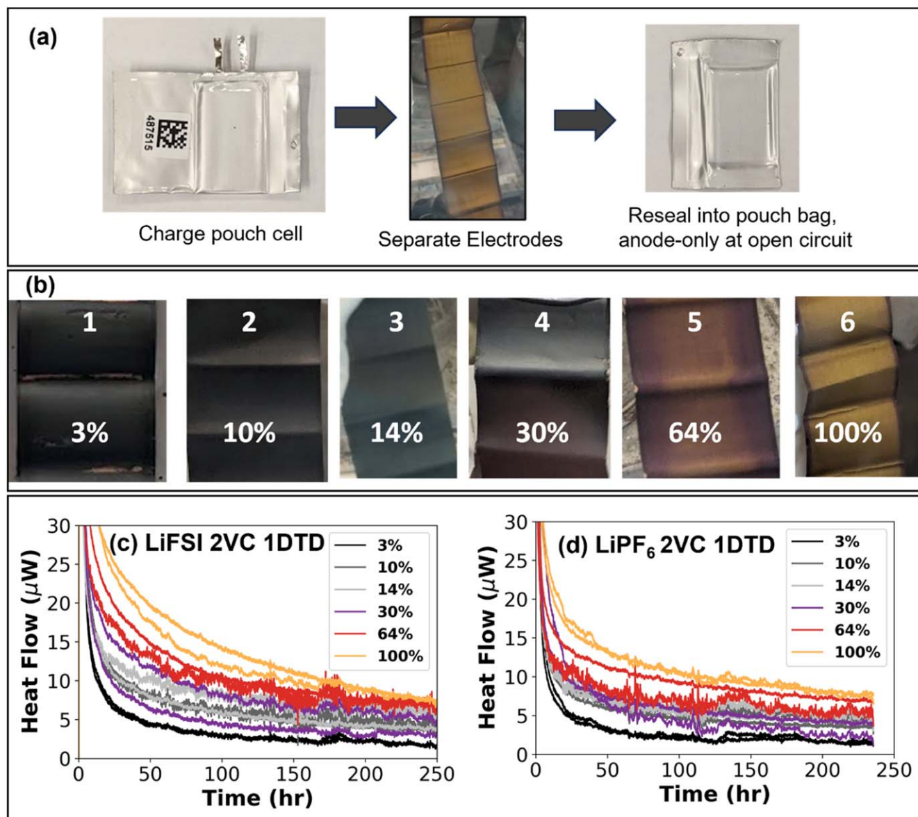
Figure 5. Isothermal microcalorimetry testing of lithiated graphite electrodes ( \text{Li}_x\text{C}_6 ) from NMC532/AG cells after formation at 40 °C. (a) Pouch bag construction procedure from lithiated negative electrodes. (b) Photographs of the extracted graphite electrodes charged to a set of 6 known states of charge, opened in an Ar-filled glovebox, with SOC labelled on each photo. Measured parasitic heat flow vs time generated from lithiated graphite reacting with electrolyte in the open circuit pouch bags, showing decay with time, with (c) LiFSI salt and (d) LiPF 6 electrolyte salts. Exothermic heat flows are shown as positive.
